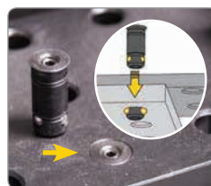
Flush Mount Ball Lock Bolts T65020
