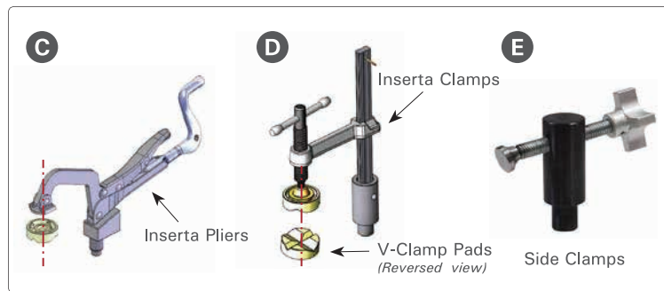
Quick hold-down clamping of flat, square, angled or round parts. Hold, stop, or locate parts using horizontal clamping force.
